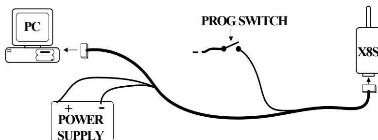
Figure 3.1 Configuration: installation
